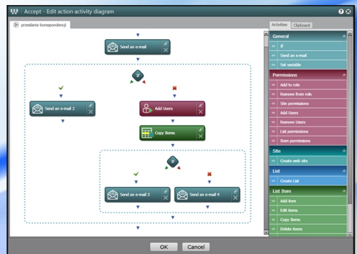
Graphical designer: activities
